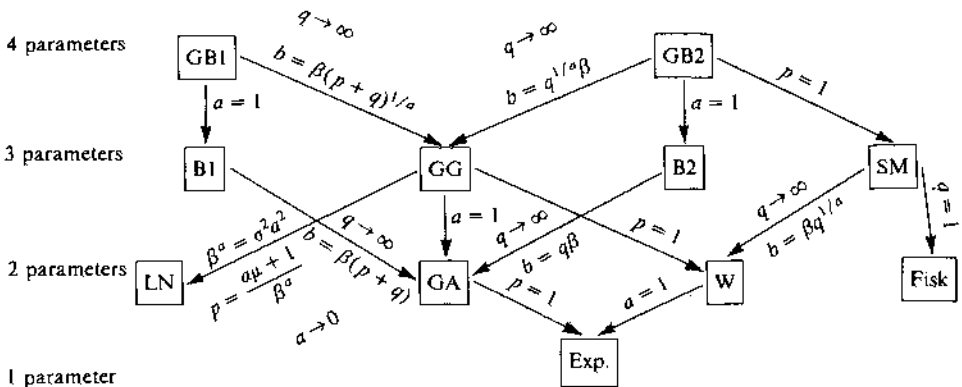
FIGURE 1—Distribution trees.
